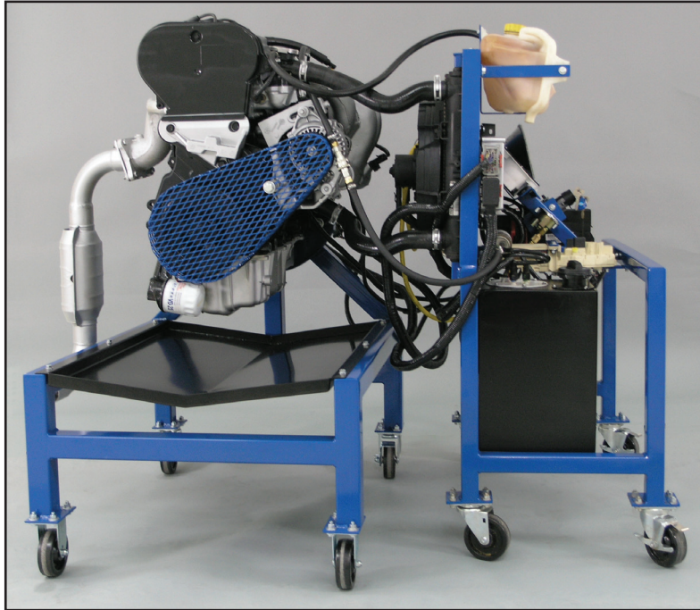
Engine Repair Trainer (model 90) connected to Engine Start Cart (model 91)
